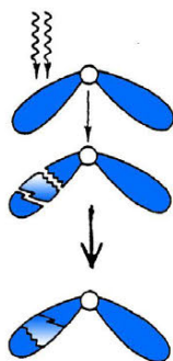
Inversion
