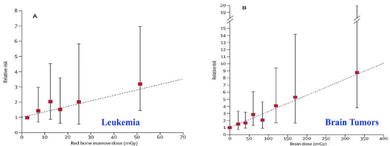
Relative risk of leukaemia and brain tumours in relation to estimated radiation doses to the red bone marrow and brain from CT scans (A) Leukaemia and (B) brain tumours. Dotted line is the fitted linear dose-response model (excess relative risk per mGy). Bars show 95% CIs.
